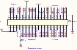
Expansion header
