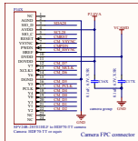
Camera FPC connector
